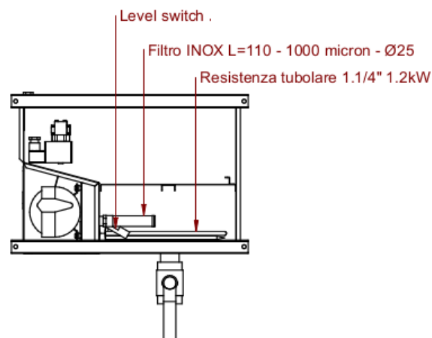
2 - Tank
